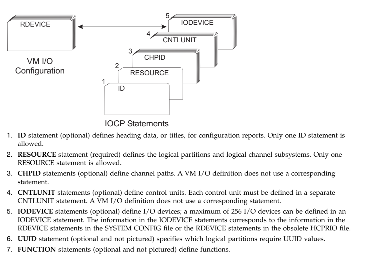
Figure 17. Correspondence between IOCP statements and SYSTEM CONFIG statements or HCPRIO statements
