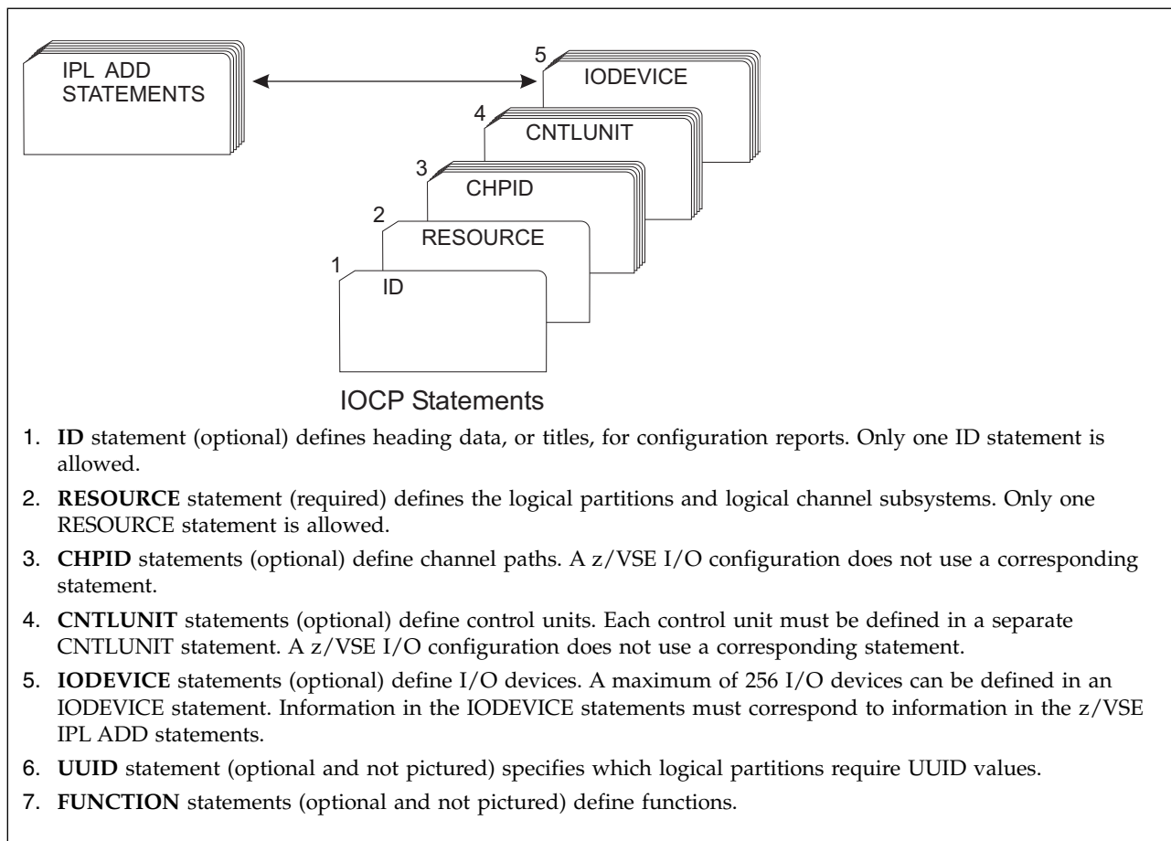
Figure 18. Correspondence between IOCP statements and z/VSE IPL ADD statements
