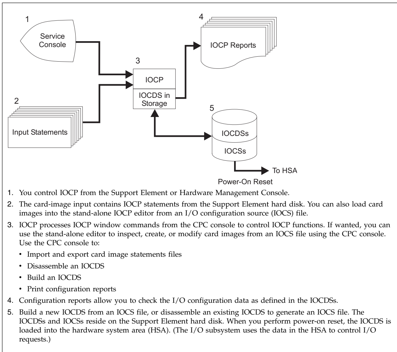
Figure 15. Overview of stand-alone version of IOCP
